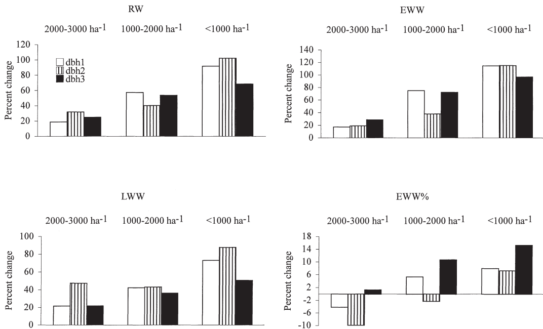
Fig. 2. Ring width (RW), early wood and late wood widths (EWW, LWW) and the percentage of early wood at given diameter classes in the stand density classes over the whole 12-year period after the thinning.
