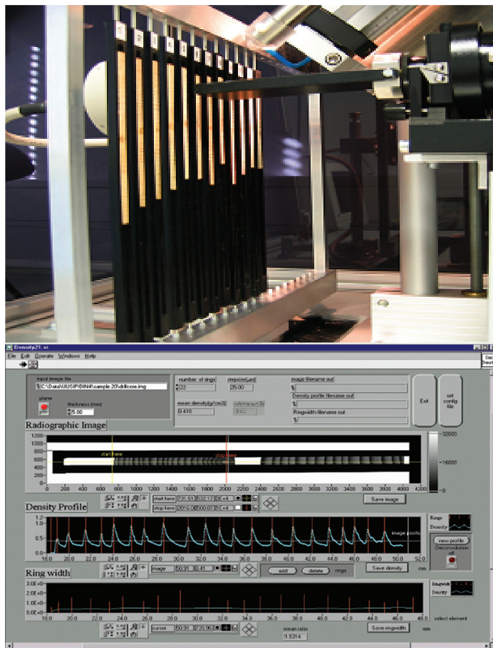
Fig. 1. X-ray microscopy (ITRAX) developed by Cox Analytical Systems (above) and a digital radiographic image and wood density profile for one example sample under analyses in Density software (below).
