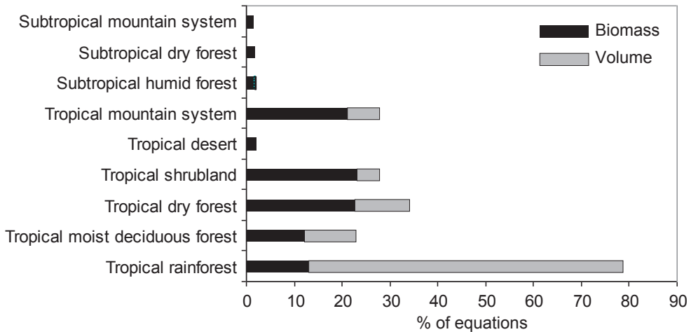
Fig. 4. Distribution of volume and biomass equations in the FAO ecological zones.
