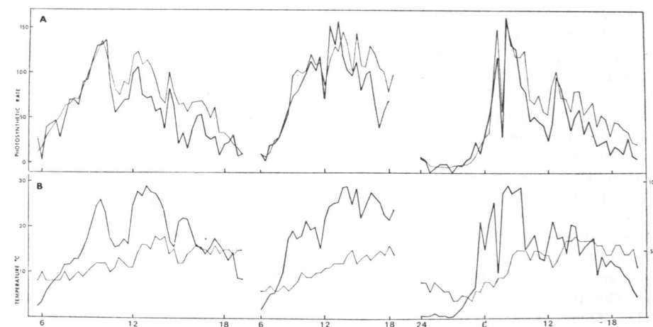
Fig. 9. A. Measured (thick line) and according Eq. (12) computed photosynthetic rates during the period 1974-06-06, 06-07 and 06-10 for Scotch pine.
