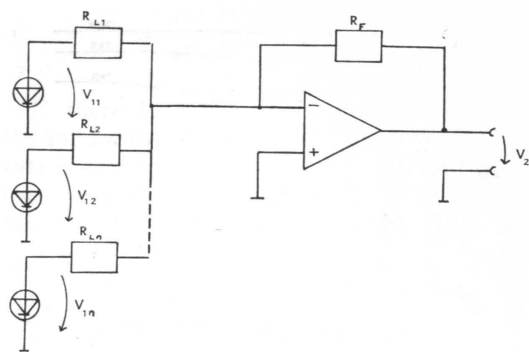
Fig. 5. The circuit diagram of the summing amplifier.
