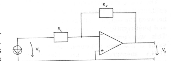
Fig. 4. The circuit diagramme of the inverting amplifier for one photovoltaic cell.
