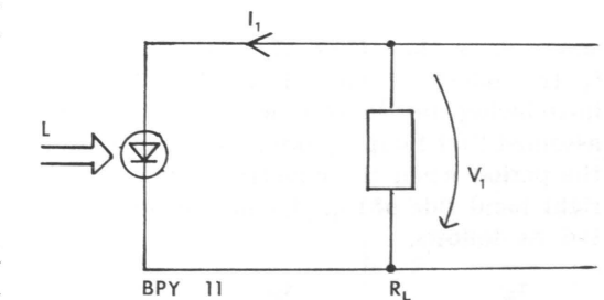
Fig. 1. The test circuit for the photo-voltaic cell BPY 11.
