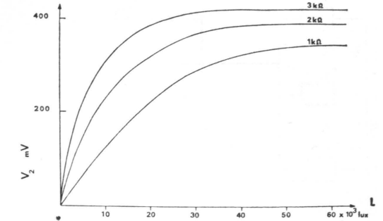
Fig. 3. The dependence of the output of the BPY 11 as function of illumination with both resistances 1 k\Omega , 2 k\Omega , 3 k\Omega .
