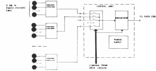
Fig. 2. The block diagramme of the ELP.
