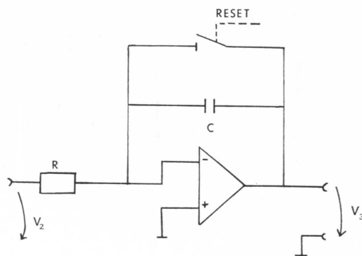
Fig. 6. Simplified diagram of the analog integrator.
