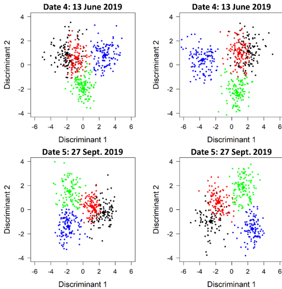
Figure S7. Class separation by two discriminant axes in the kappa-optimized tree species classification by multispectral-based and RGB-based segmentations on the five inventoried dates.
