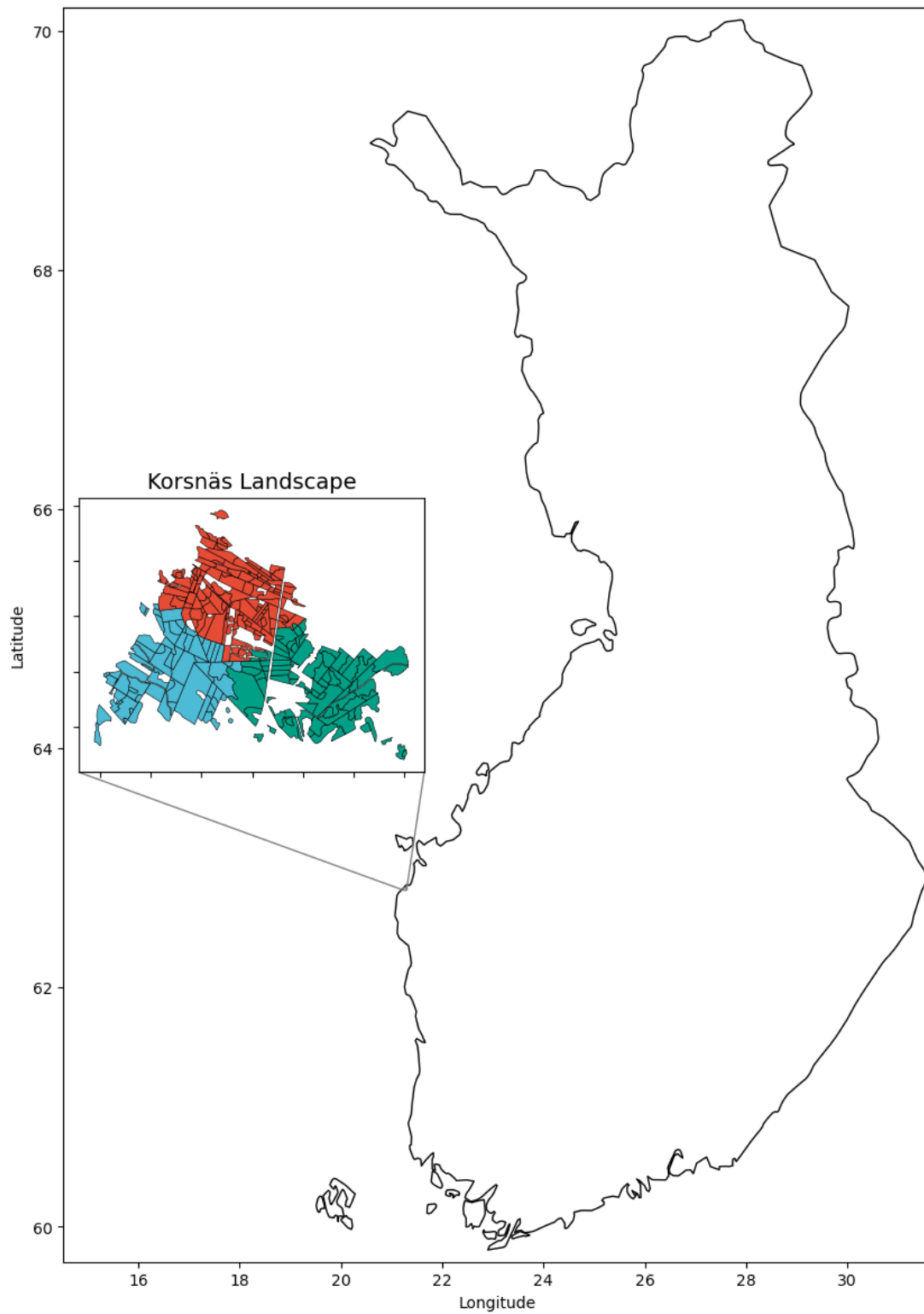
The case study landscape. The three colors represent the regions where selected wind disturbance occurs.
